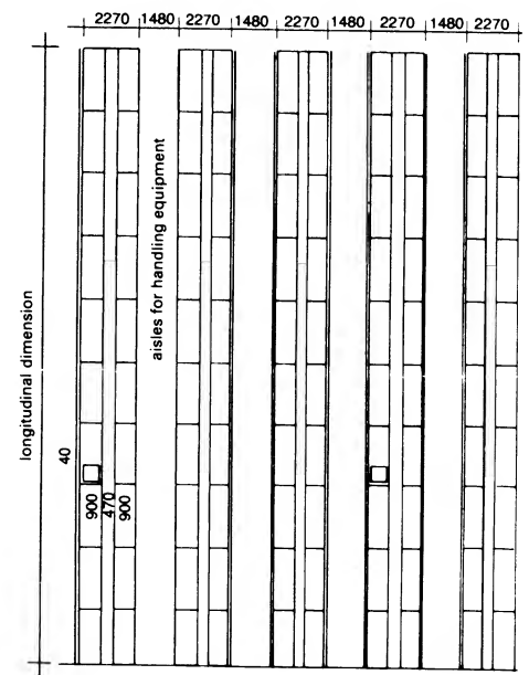
⑫ Detail of a plan for a pallet rack store for ball bearings (structural elements of shed concealed in shelving)
